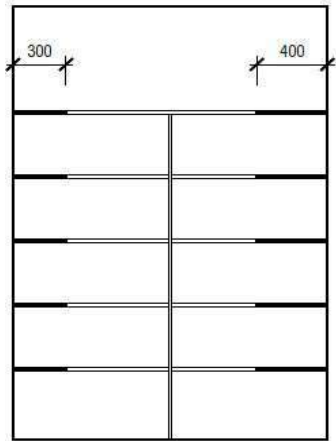
Typical 5No shelf Pantry and Linen - white melamine finish.
